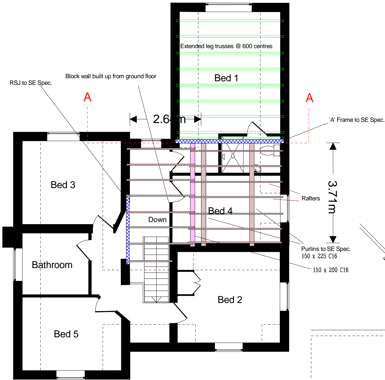
First Floor - Proposed Roof Structure (Subject to SE and truss manufacturer confirmation)
